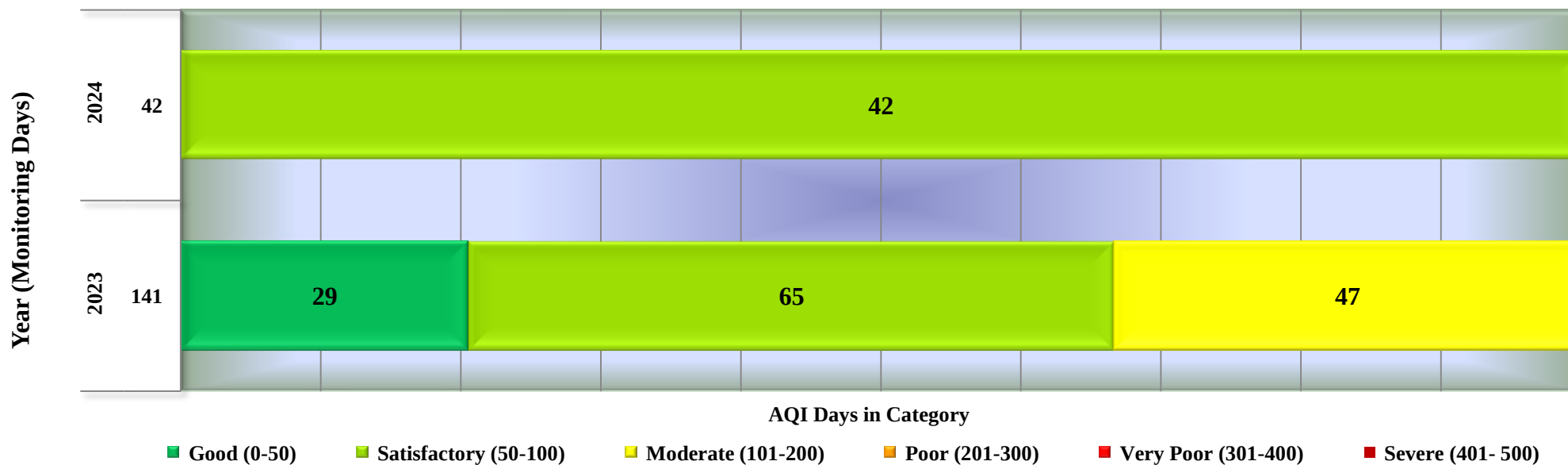
Days in various AQI categories of Indore, Vijay Nagar (Year 2023 - 2024)
