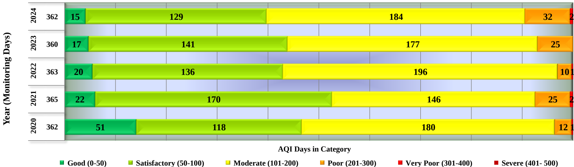
Days in various AQI categories of Pithampur, Sec-2 Industrial Area (Year 2020 - 2024)
