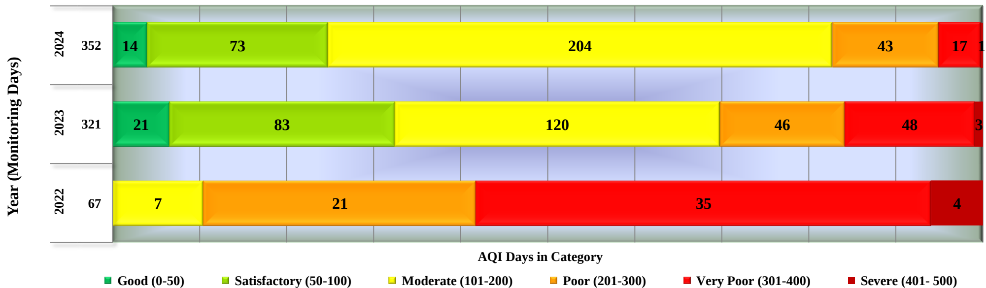
Days in various AQI categories of Gwalior, Maharaj bada (Year 2022 - 2024)
