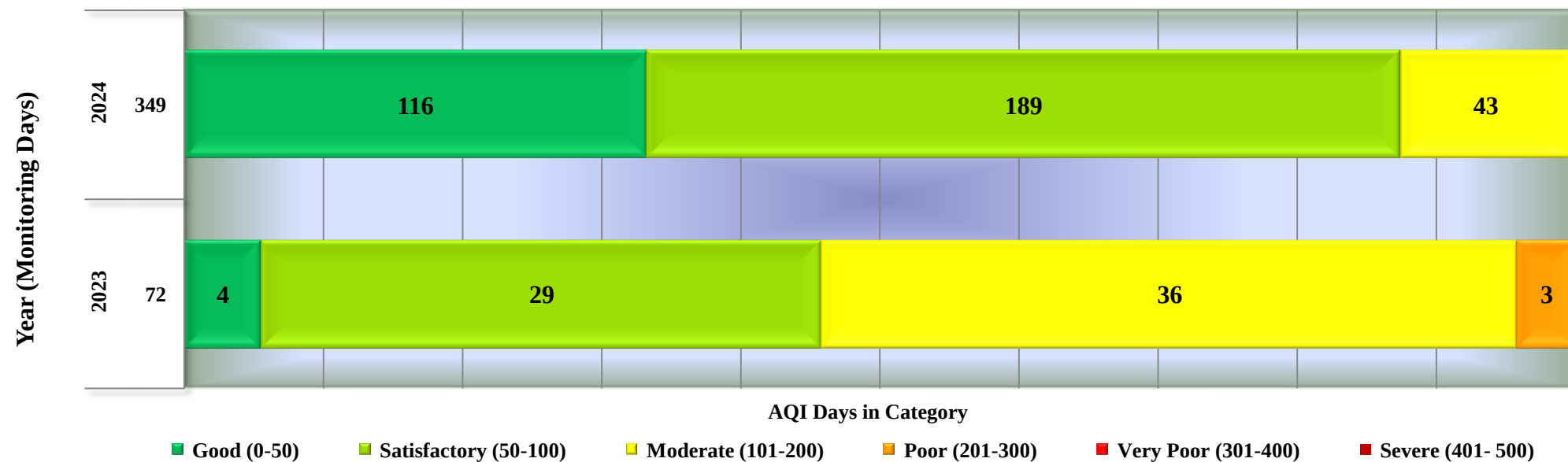
Days in various AQI categories of Indore, Residency Area (Year 2023 - 2024)
