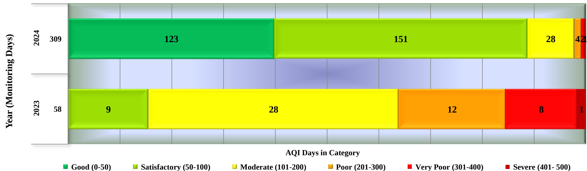
Days in various AQI categories of Indore, Maguda Nagar (Year 2023 - 2024)
