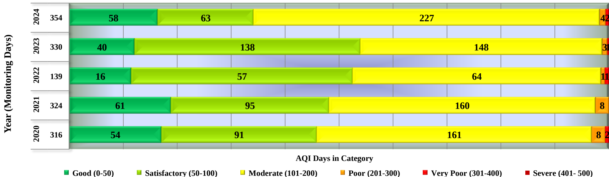
Days in various AQI categories of Ratlam, Shathri Nagar (Year 2020 - 2024)
