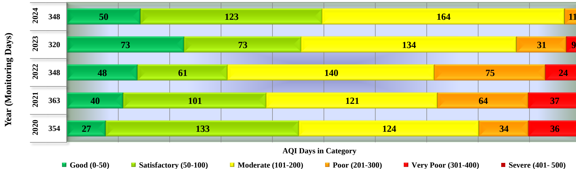
Days in various AQI categories of Katni, Gole Bazar (Year 2020 - 2024)
