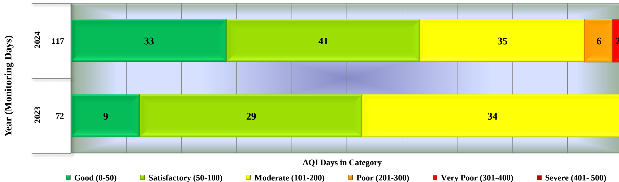
Days in various AQI categories of Indore, Airport Area (Year 2023 - 2024)
