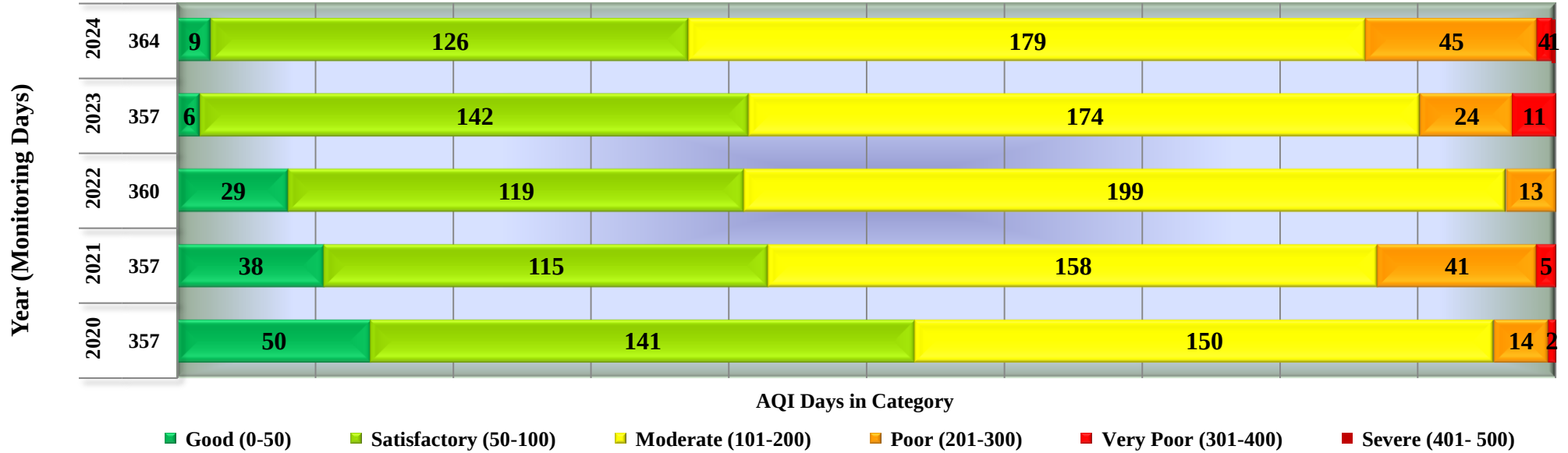
Days in various AQI categories of Indore, Chhoti Gwaltoli (Year 2020 - 2024)
