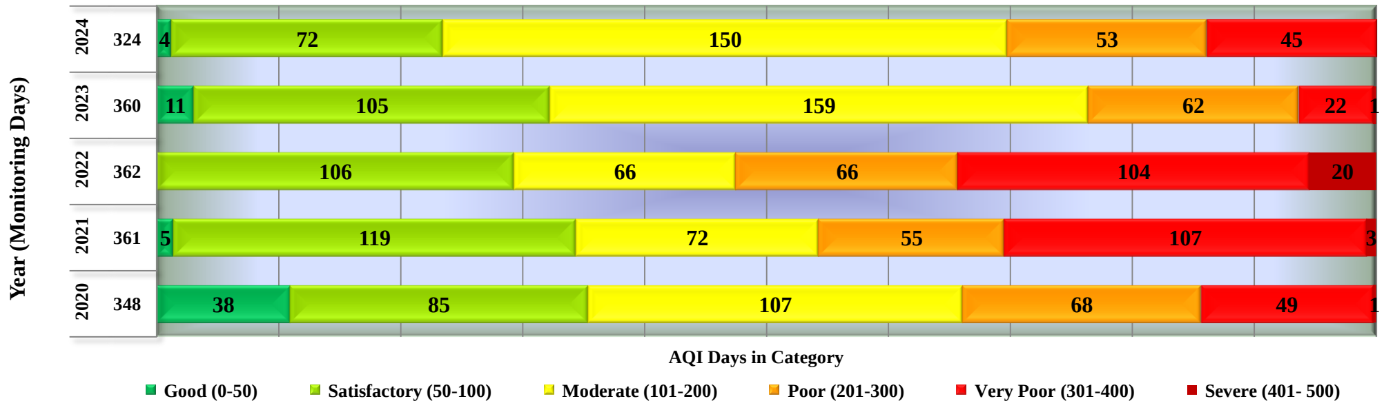
Days in various AQI categories of Singrauli, Surya Kiran Bhawan (Year 2020 - 2024)
