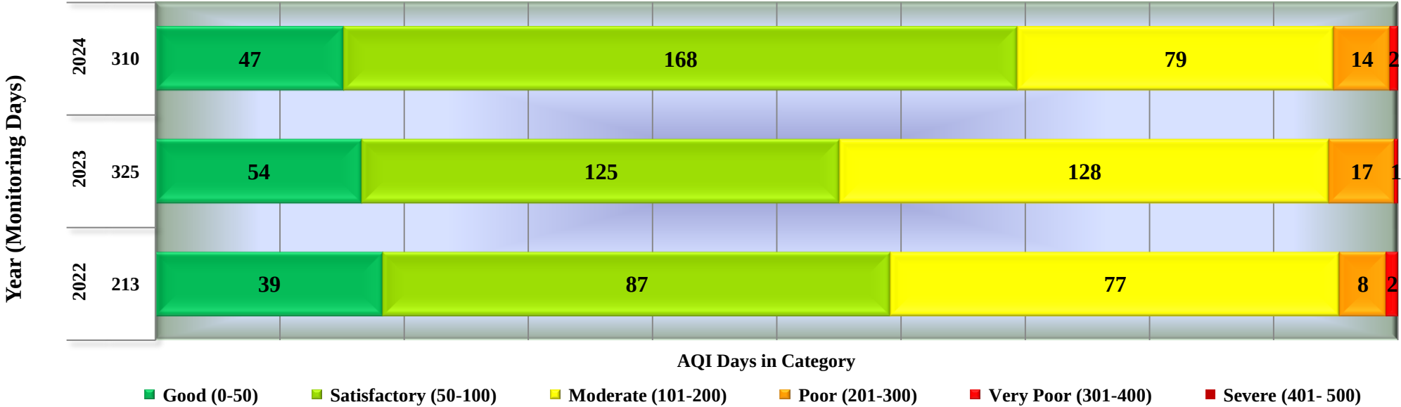
Days in various AQI categories of Dewas, Govt. MG Hospital (Year 2022 - 2024)
