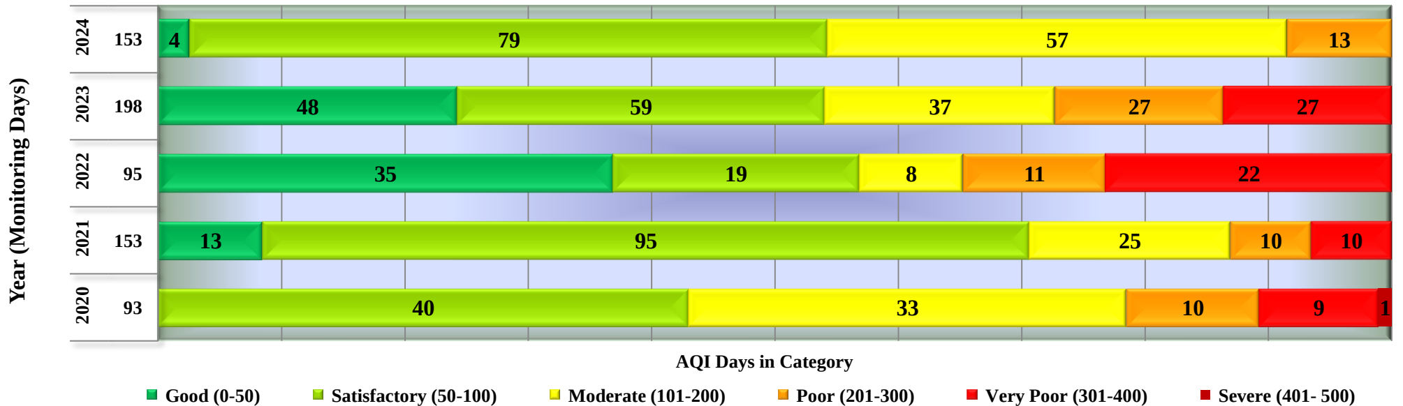
Days in various AQI categories of Gwalior, Phool Bagh (Year 2020 - 2024)
