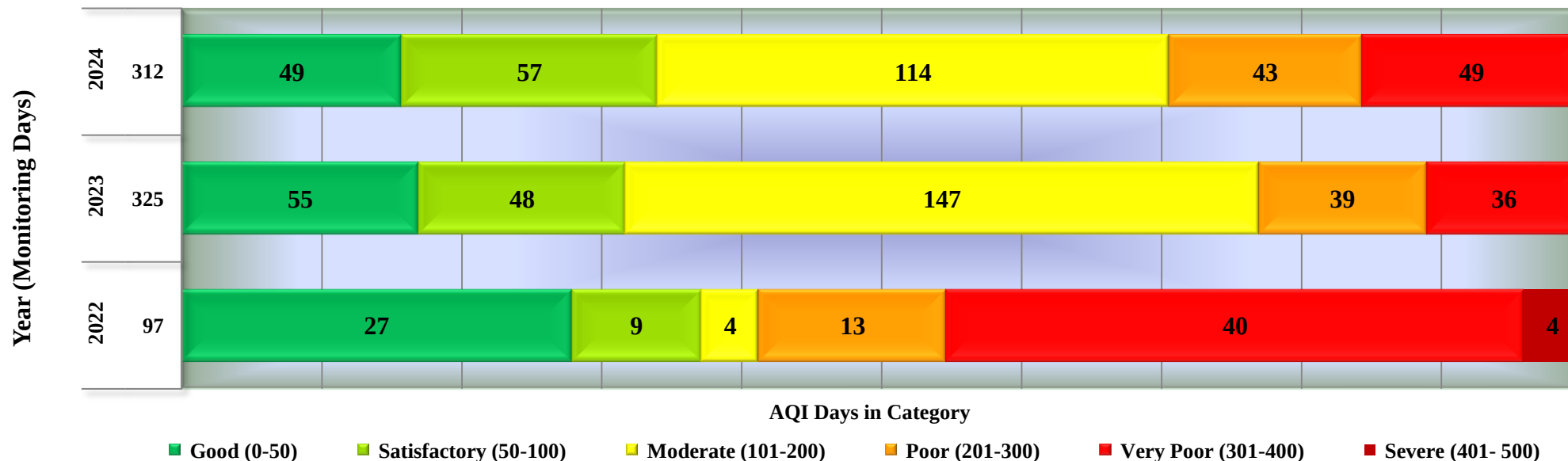
Days in various AQI categories of Singrauli, Trauma Centre Waidhan (Year 2022 - 2024)
