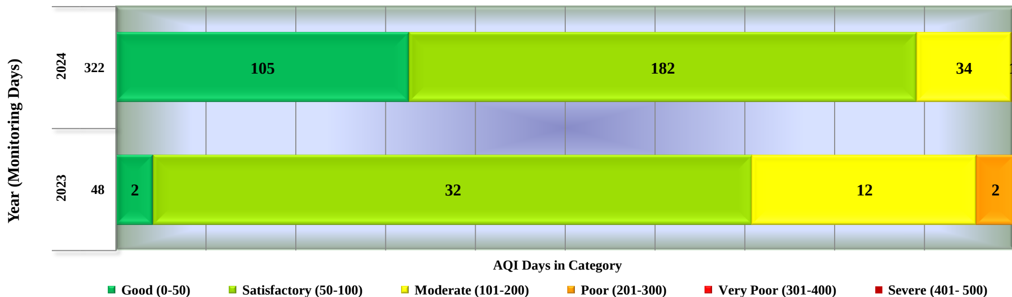
Days in various AQI categories of Indore, Regional Park N Nigam (Year 2023 - 2024)
