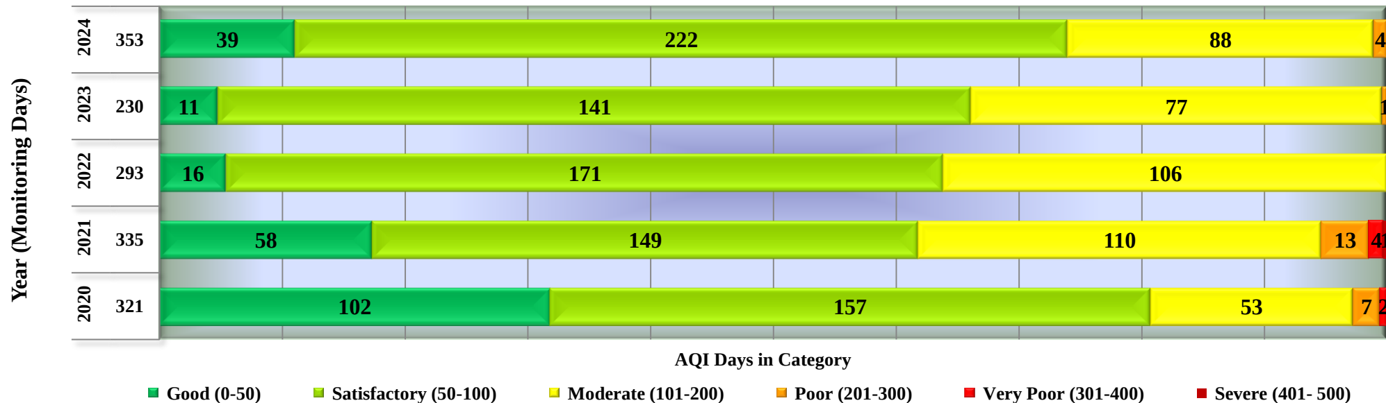
Days in various AQI categories of Sagar, Deen Dayal Nagar (Year 2020 - 2024)
