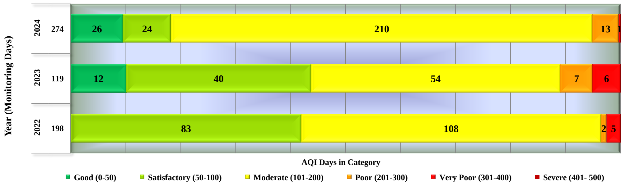
Days in various AQI categories of Betul , Collector Office (Year 2022 - 2024)
