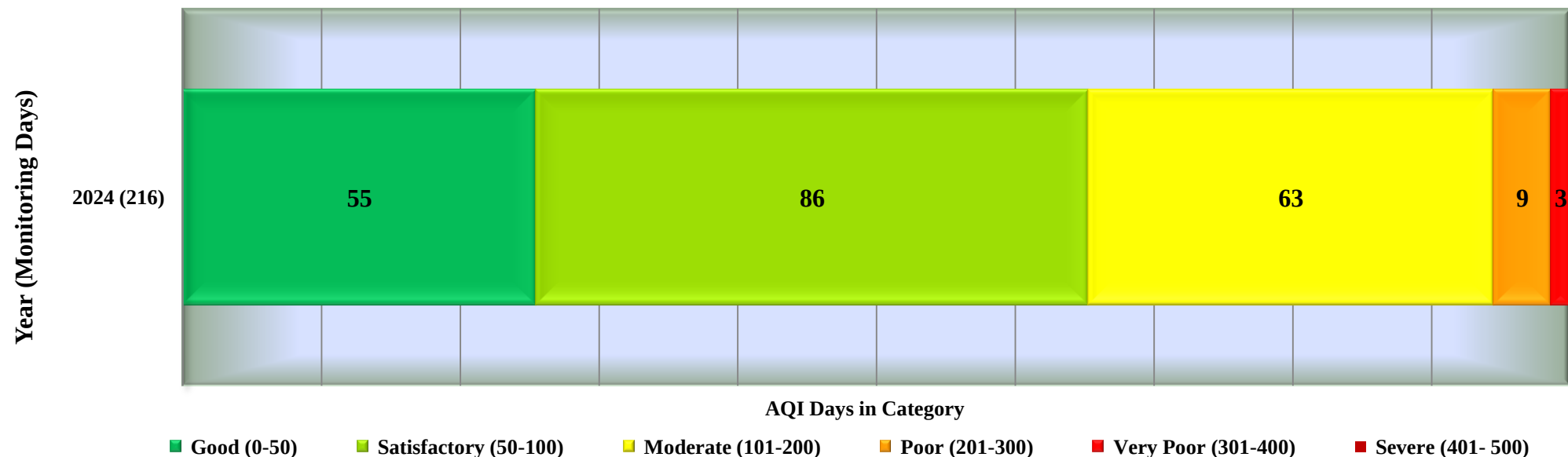
Days in various AQI categories of Jabalpur, Gupteshwar (Year - 2024)
