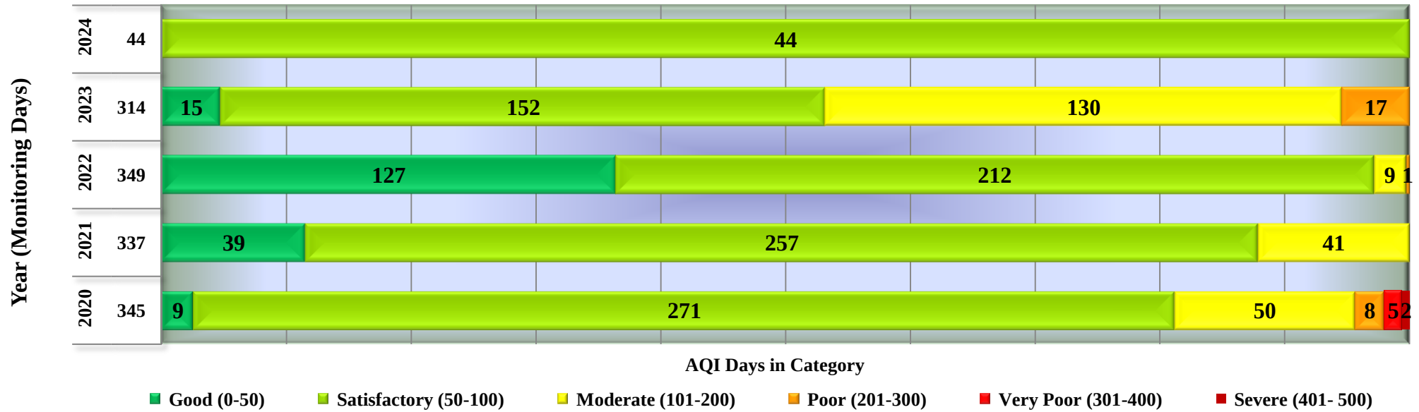
Days in various AQI categories of Satna, Bandhavgar Colony (Year 2020 - 2024)
