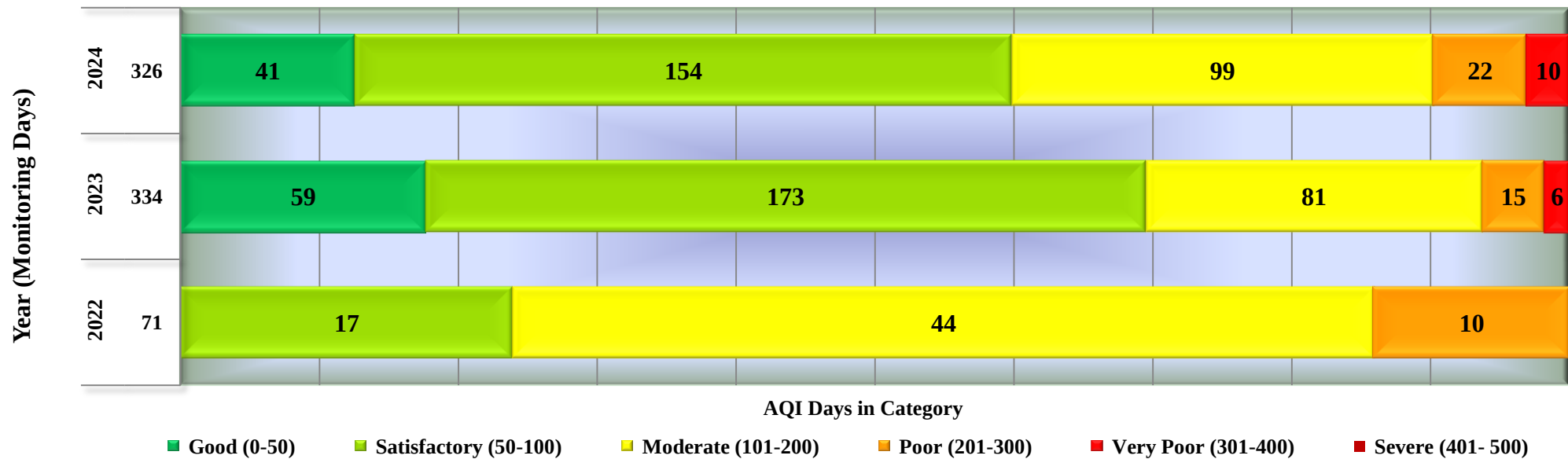
Days in various AQI categories of Sagar, Collectorate Office (Year 2022 - 2024)
