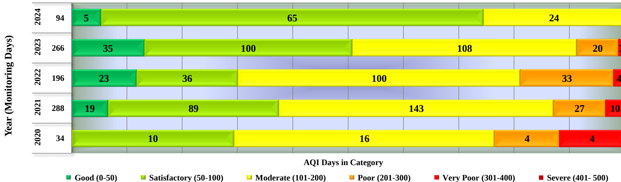
Days in various AQI categories of Katni, Regional Office (Year 2020 - 2024)
