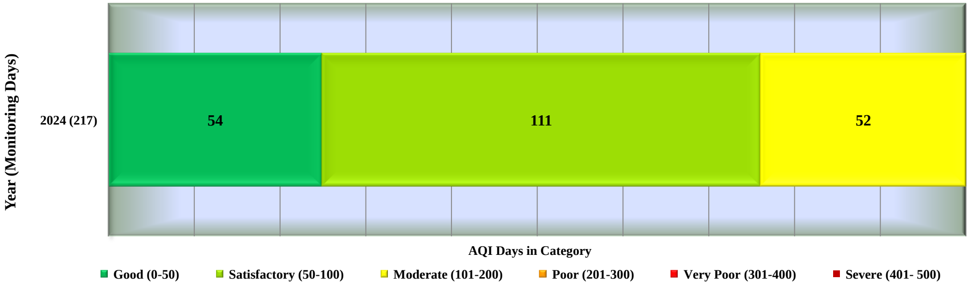
Days in various AQI categories of Indore, Pologround (Year - 2024)
