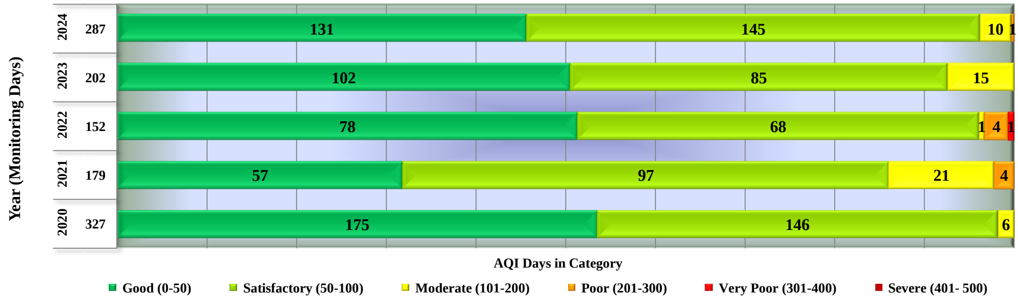
Days in various AQI categories of Maihar , Sharda Temple (Year 2020 - 2024)
