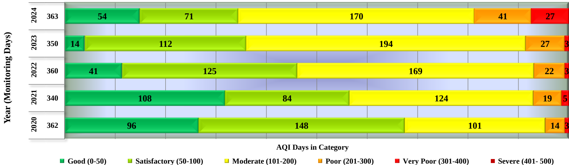
Days in various AQI categories of Mandideep, Industrial Area (Year 2020 - 2024)
