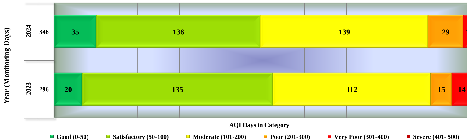
Days in various AQI categories of Bhopal, Collectorate Office (Year 2023 - 2024)
