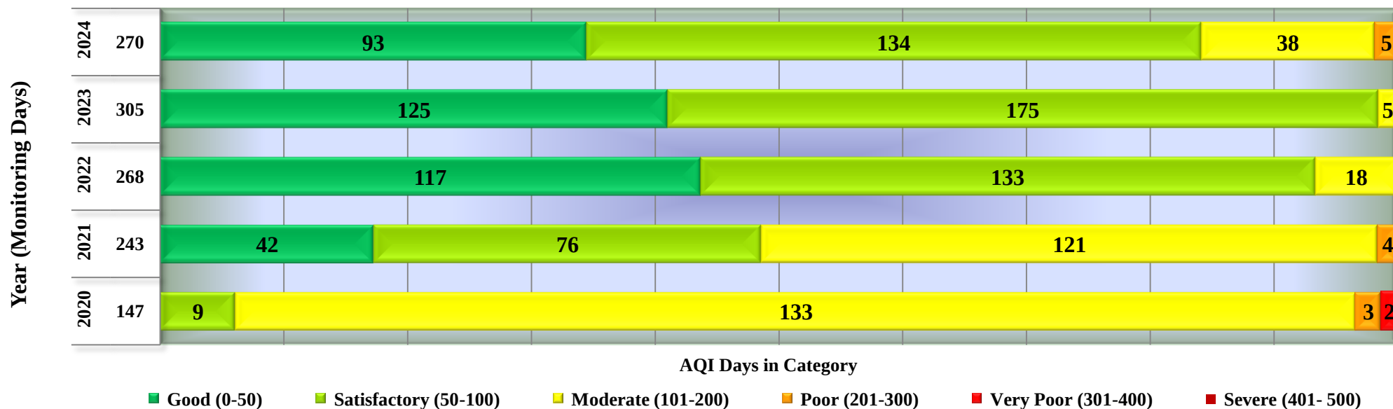
Days in various AQI categories of Anuppur, Collectorate (Year 2020 - 2024)
